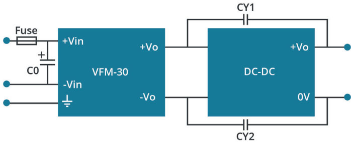
Figure 1 Application Circuit
