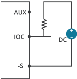
Figure 10 External DC Power
