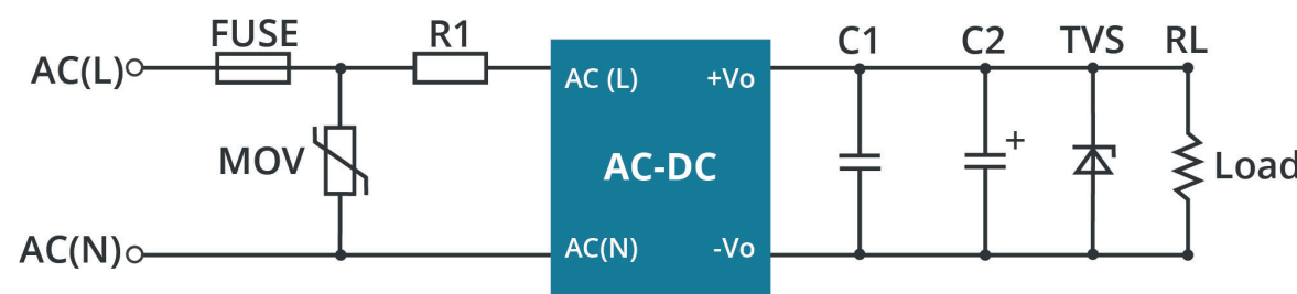
Figure 2 EMC APPLICATION CIRCUIT WITH HIGHER REQUIREMENTS
