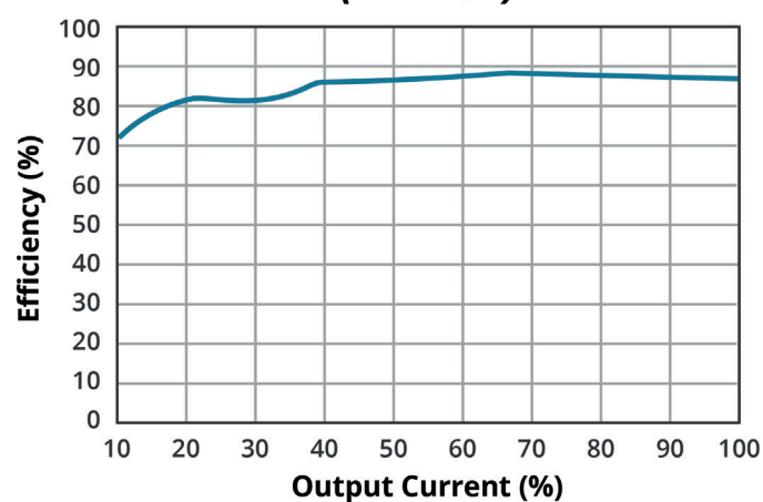
EFFICIENCY VS OUTPUT LOAD ( V_{in} = 48V )
