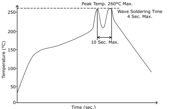
Wave Soldering Profile
