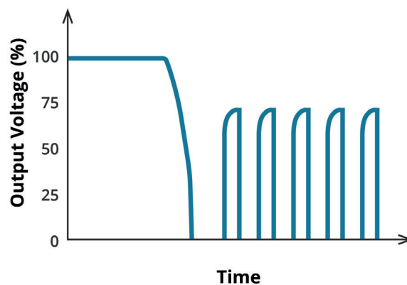
OUTPUT VOLTAGE VS TIME HICCUP MODE
