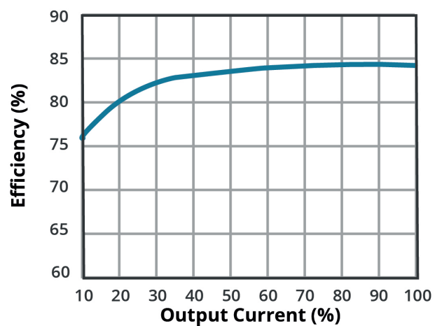
EFFICIENCY VS OUTPUT LOAD AE40-EW-S15-T
