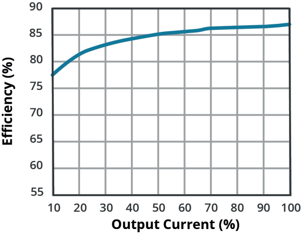
EFFICIENCY VS OUTPUT LOAD AE40-EW-S24-T
