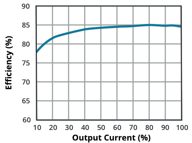
EFFICIENCY VS OUTPUT LOAD AE40-EW-S12-T
