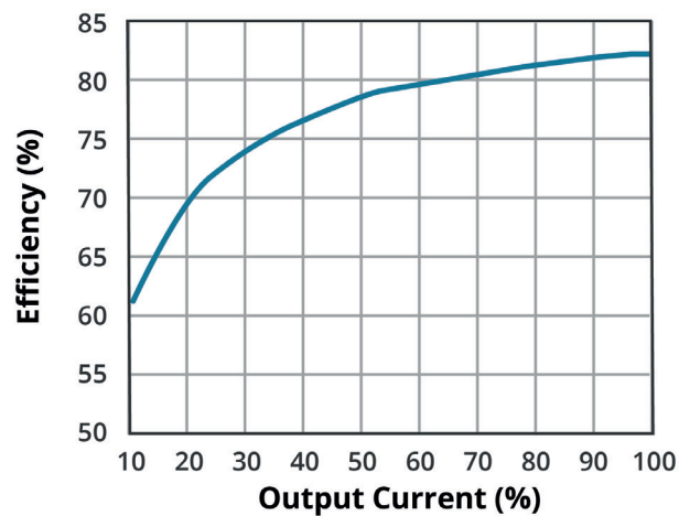
EFFICIENCY VS OUTPUT LOAD AE10-EW-S24
