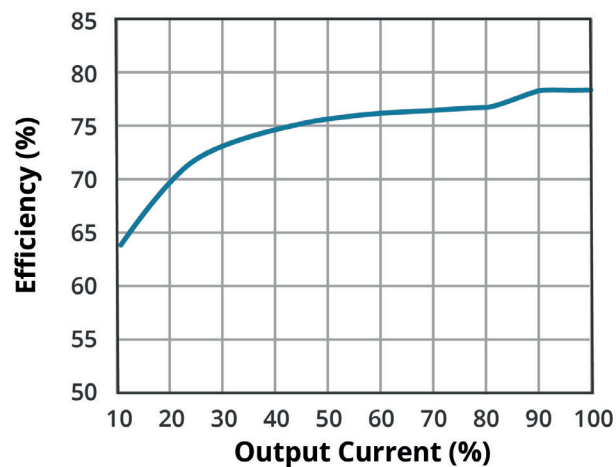
EFFICIENCY VS OUTPUT LOAD AE10-EW-S9
