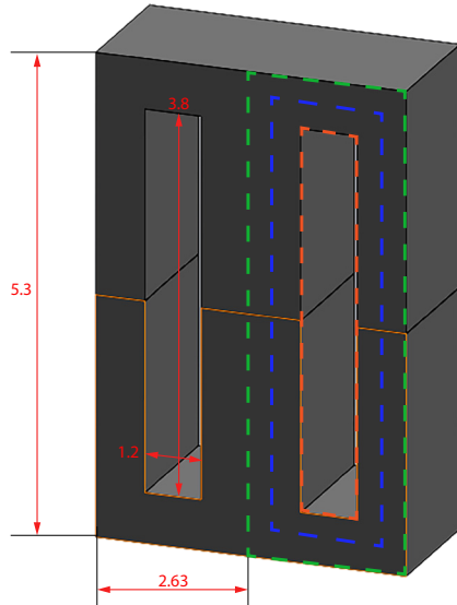
EE CORE
