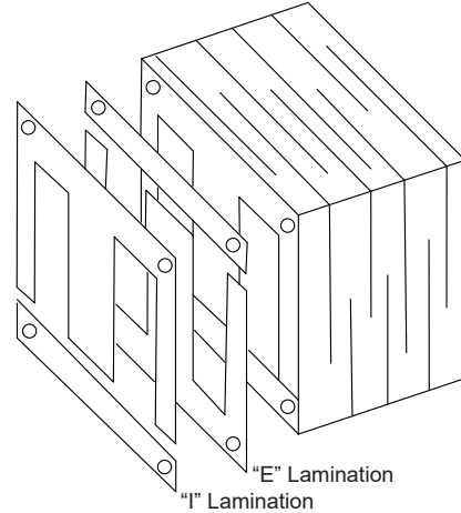
LAMINATED CORE
