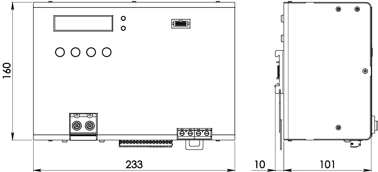
Figure 2. Mechanical Drawing
