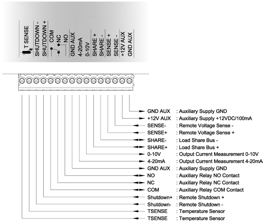
Figure 1. Auxiliary connector
