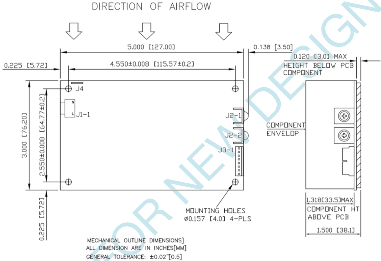
Figure 2. Mechanical Drawing
