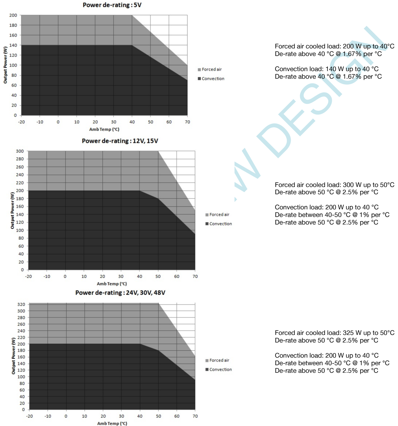
Figure 1. Derating Curves
